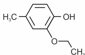
2-ethoxy-4-methylphenol
