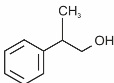
2-phenylpropan-1-ol
