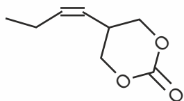
Hex-3-en-1-yl methyl carbonate
