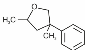
2,4-dimethyl-4-phenyloxolane
